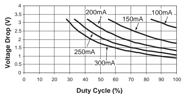
Device Duty Cycle vs. V_{DROP} ( V_{DROP} = 2.8\text{V} @ 85^\circ\text{C} )
