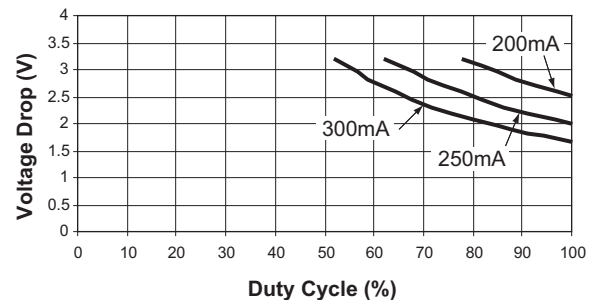
Device Duty Cycle vs. V_{DROP} ( V_{DROP} = 2.8\text{V} @ 85^\circ\text{C} )
