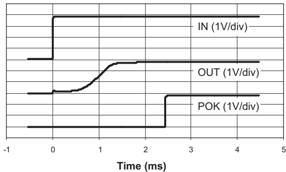
Power-Up With 100mA Load
