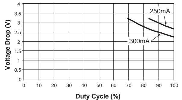
Device Duty Cycle vs. V_{DROP} ( V_{DROP} = 2.8\text{V} @ 50^\circ\text{C} )
